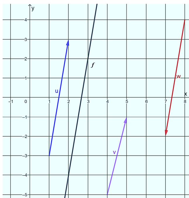
Figure 3: Collinear Vectors
