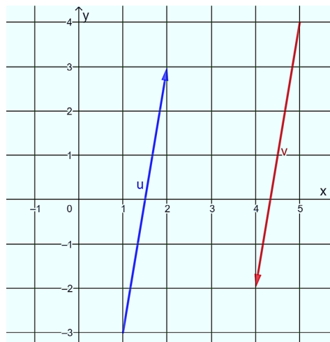
Figure 4: Negative Vectors
