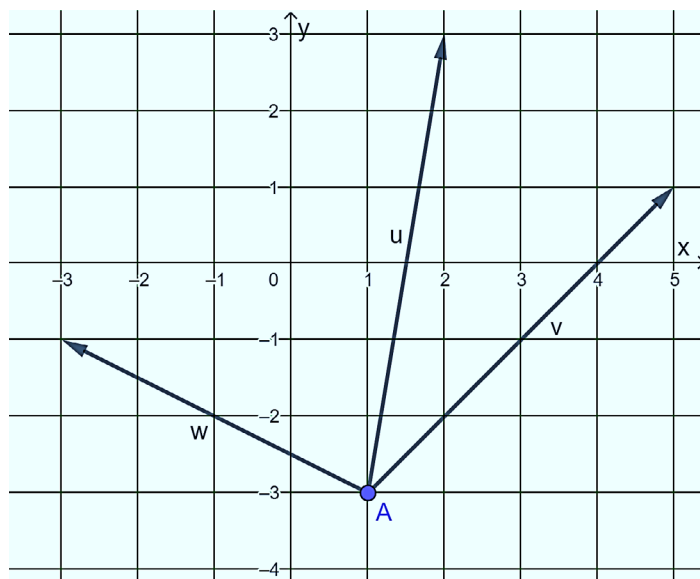
Figure 2: Co-initial Vectors
