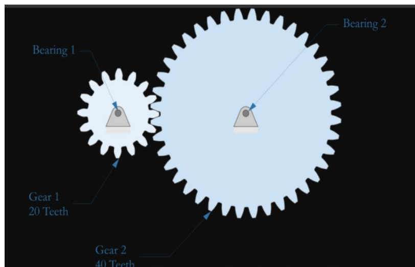
Fig. 19.4: Diagram showing Gear 1 with 20 teeth and Gear 2 with 40 teeth
