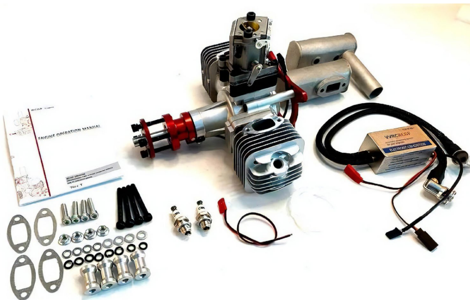
Figure 11: A gas engine kit for radio-controlled aircraft
