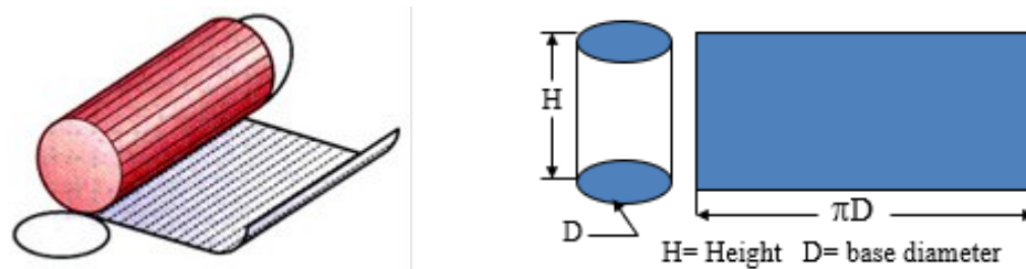
Fig. 10.1: Development of a cylinder using parallel line method.
