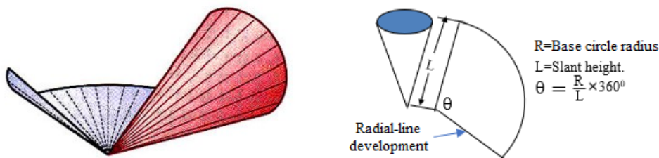
Fig. 10.2: Development of a cone using radial line method
