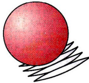
Fig. 10.4: Development of a sphere using approximate method
