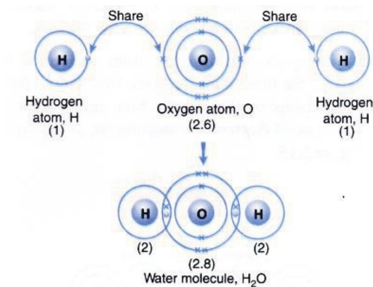
Fig. 2.12: Formation of molecule of water
