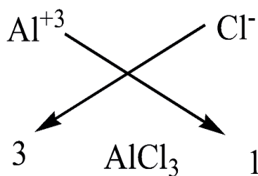
Fig. 2.17: Formation of Aluminium chloride
