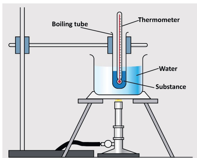
Fig 1.1: Boiling point of water
