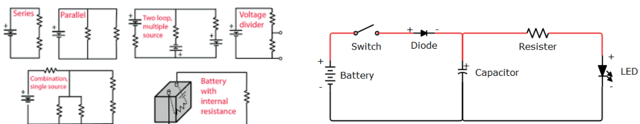
Fig. 12.4: Different Analogue Circuits
