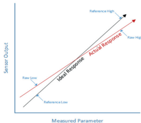
Fig. 8.1: Two-point Calibration.
