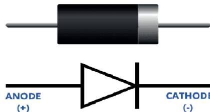
Fig. 9.4: An actual Diode and the symbol for a diode
