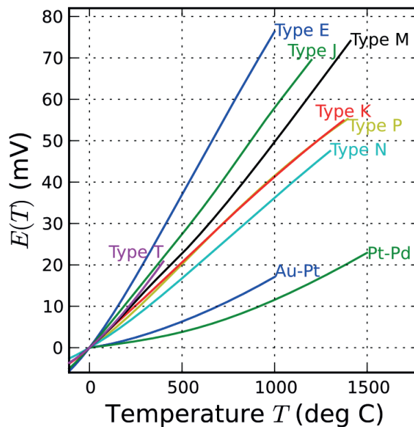
Fig. 7.3 Thermocouple functions
