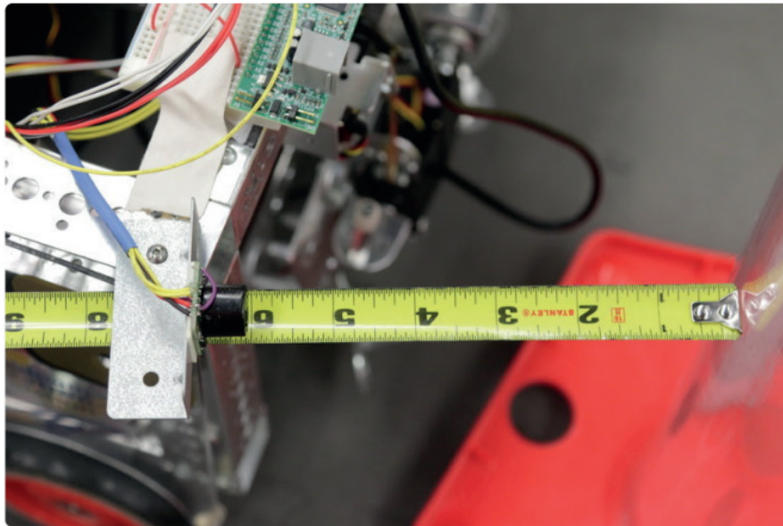
Fig. 7.5: One-point calibration
