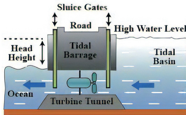
Figure 74: A picture of how tidal energy is generated
