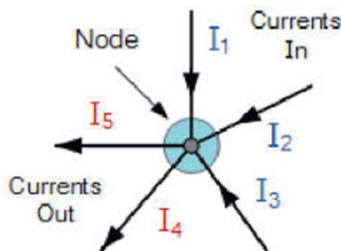
Figure 46: A picture illustrating KCL
